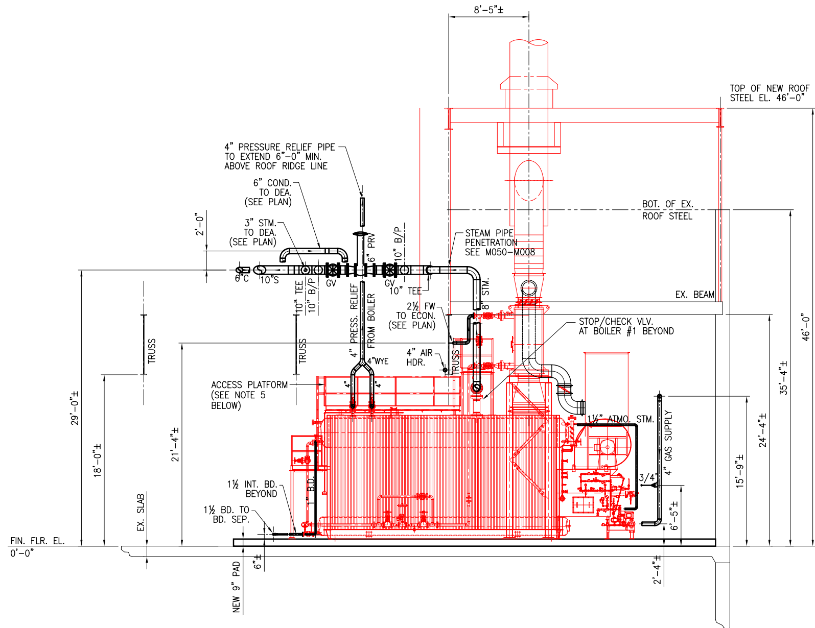
SECTION C SCALE: 3/16"=1'-0" M003
